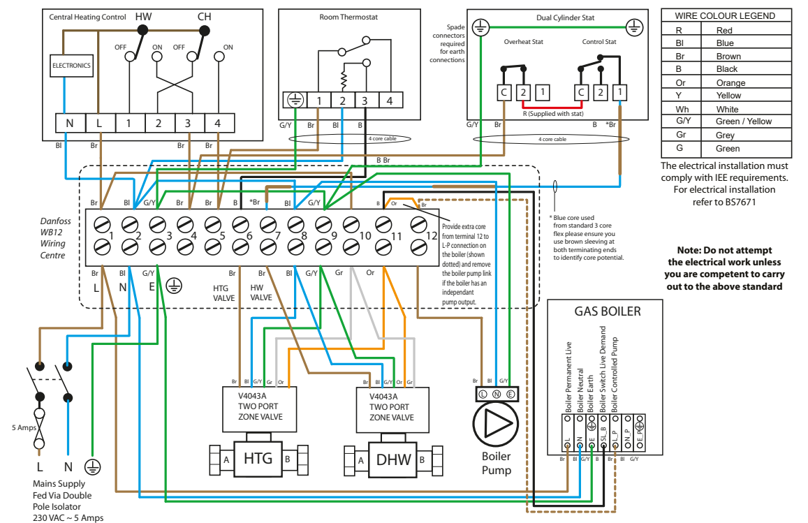
Typical schematic wiring diagram for an unvented installation
