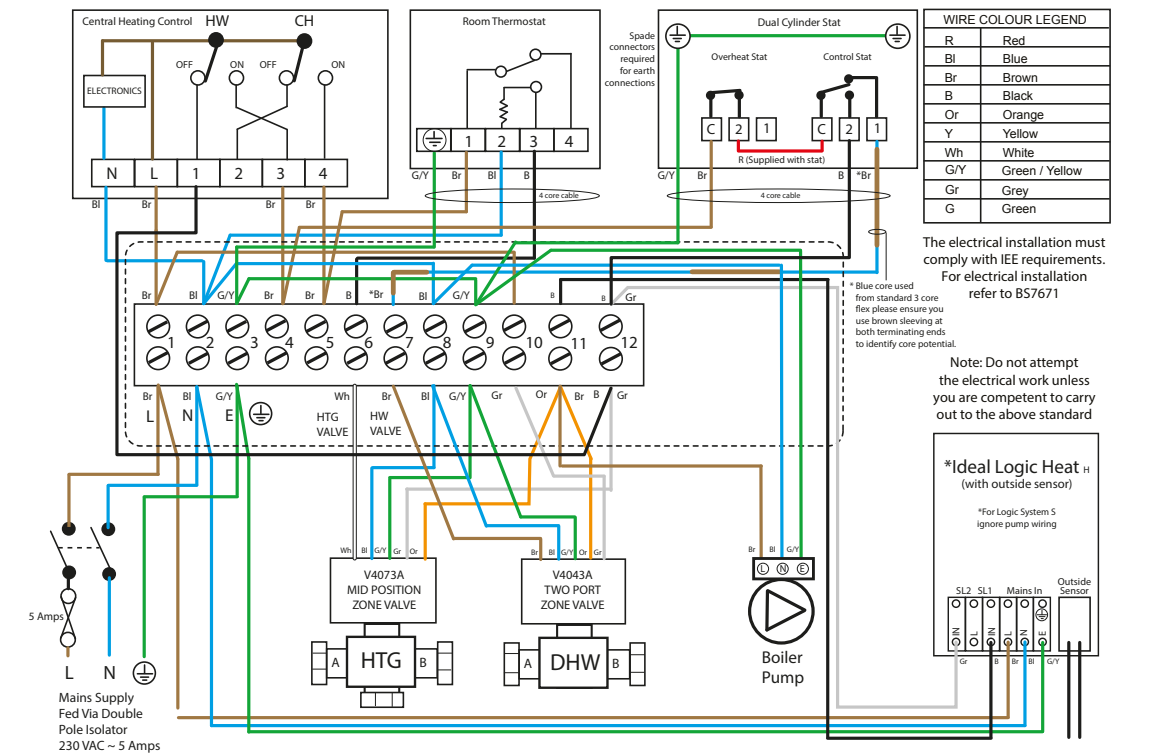
Ideal schematic wiring diagram for an unvented installation
